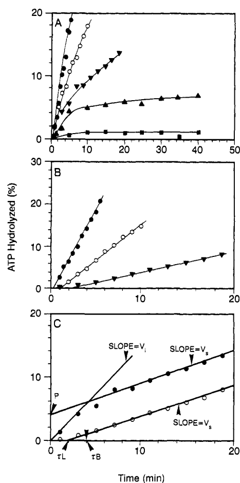
FIGURE 1: Effect of ADP on the kinetics of poly(dT)-dependent ATP hydrolysis. The amount of ATP hydrolyzed at different times was measured in the presence of ADP with two different orders of addition. The concentrations of recA protein, poly(dT), and ATP are 5 \mu M, 10 \mu M, and 2 mM, respectively. (A) RecA protein and poly(dT) were preincubated for 10 min, and then the reaction was initiated with a mixture of ATP and ADP. Concentrations of ADP were as follows: 0 ( \bullet ), 1 ( \circ ), 2 ( \nabla ), 3 ( \blacktriangle ), and 4 ( \blacksquare ) mM. (B) RecA protein, poly(dT), and ADP were preincubated for 10 min, and then ATP was added to initiate the reaction. Concentrations of ADP were as follows: 0 ( \bullet ), 1 ( \circ ), and 2 ( \nabla ) mM. (C) Comparison of burst and lag type kinetics at an ADP/ATP ratio = 1.0. The variables used are as follows: the time intercept ( \tau ), the amplitude of the burst ( P ), the initial velocity ( V_i ), and the steady-state velocity ( V_s ). Conditions are identical with those in panels A and B, except that ATP and ADP are both 2 mM. Lines defined by ( \bullet ) and ( \circ ) reflect the protocols of panels A and B, respectively.
