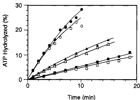
FIGURE 8: Effect of ADP on high-salt-activated (DNA-independent) ATP hydrolysis. ATP hydrolysis was measured in the presence of ADP with two different orders of addition of nucleotides. First, recA protein was preincubated for 10 min, and then a mixture of ATP and 1 ( \circ ), 3 ( \Delta ), or 6 ( \square ) mM ADP was added to initiate the reaction. Second, recA protein and 1 ( \bullet ), 3 ( \blacktriangle ), or 6 ( \blacksquare ) mM ADP were preincubated for 10 min, and then ATP was added to initiate the reaction. The concentrations of recA protein and ATP were 5 \mu M and 2 mM, respectively.
