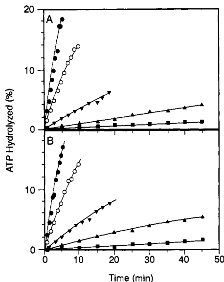
FIGURE 7: Effect of the length of poly(dT) on the transient phase. Shorter DNA [(dT) 60 ] was used. Concentrations of recA protein, (dT) 60 , and ATP are 6 \mu M, 10 \mu M, and 2 mM, respectively. (A) RecA protein was preincubated with (dT) 60 . After 10 min, a mixture of ATP and ADP was added to initiate reaction. (B) RecA protein was preincubated with (dT) 60 and ADP. After 10 min, ATP was added. In both cases, ADP concentrations were 0 ( \bullet ), 1 ( \circ ), 2 ( \blacktriangledown ), 3 ( \blacktriangle ), and 4 ( \blacksquare ) mM ADP.
