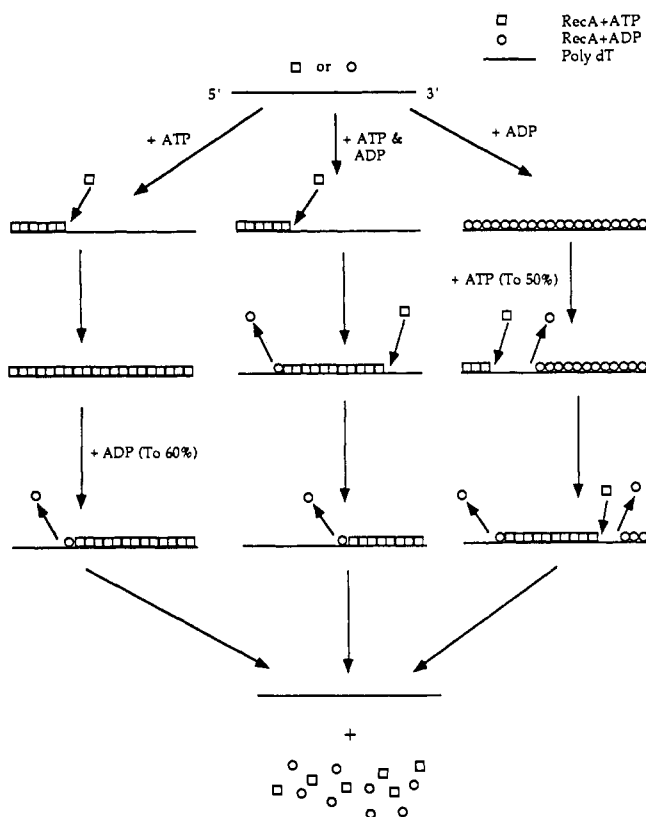
FIGURE 11: A model for recA filament assembly and disassembly mediated by ATP and ADP. The ATP- and ADP-stabilized conformations of recA protein are denoted by squares and circles, respectively. The polarity of filament assembly in the presence of ATP is that observed by Register and Griffith (1985). The polarity of assembly in the presence of ADP (if any) is unknown. The illustrated polarities of disassembly are hypothetical.
