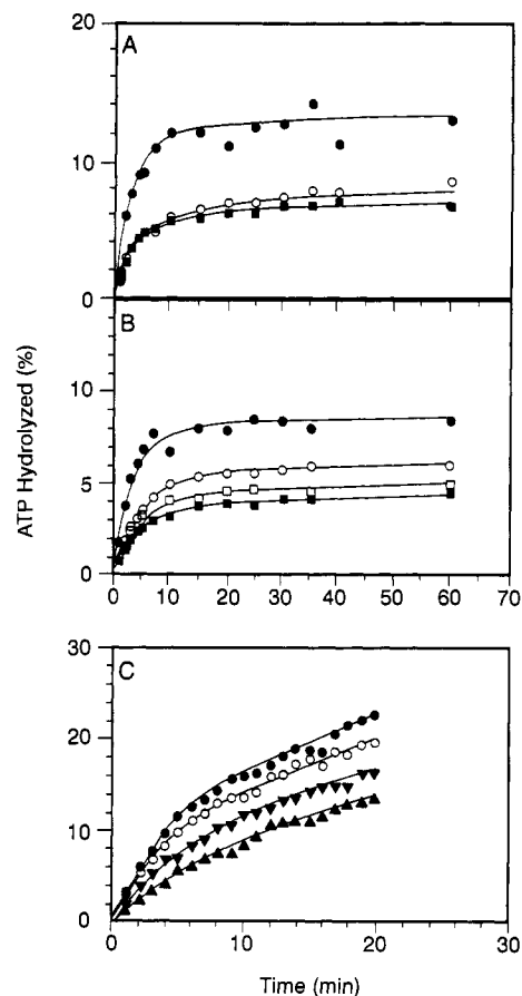
FIGURE 3: Characterization of burst kinetics: (A) Effect of recA protein and poly(dT) concentration on the amplitude of the burst at ADP/ATP = 1.5. The concentrations of ATP and ADP were 2 and 3 mM, respectively, and the order of addition protocol of Figure 1A was used. The concentrations of poly(dT) and recA protein, respectively, were as follows: (■) 10 \mu M, 5 \mu M; (○) 10 \mu M, 10 \mu M; (●) 20 \mu M, 10 \mu M. (B) Effect of order of addition on burst amplitude. RecA protein, poly(dT), ATP, and ADP concentrations were 5 \mu M, 10 \mu M, 2 mM, and 3 mM, respectively. Preincubations were for 10 min at 37 °C with components designated "pre", before initiation with components designated "I": (●) (pre) poly(dT) and recA, (I) ATP and ADP; (○) (pre) recA and ATP, (I) poly(dT) and ADP; (□) (pre) recA, (I) poly(dT), ATP, and ADP; (■) (pre) recA and ATP and ADP, (I) poly(dT). (C) Effect of recA protein concentration on burst kinetics at 2 (▲), 5 (▼), 10 (○), and 20 (●) \mu M recA protein and at an ADP/ATP ratio of 1.0. Concentrations of poly(dT), ATP, and ADP are 10 \mu M, 2 mM, and 2 mM, respectively, and the order of addition protocol is that of Figure 1A.
