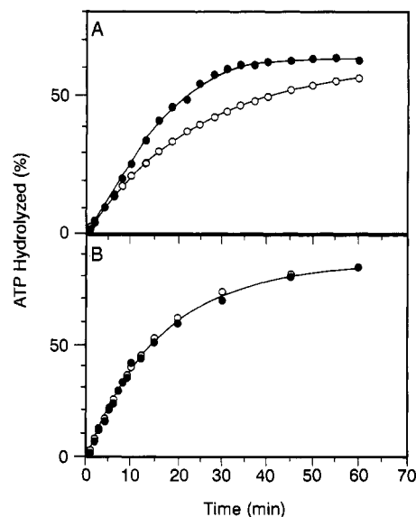
FIGURE 9: Comparison of experimental theoretical values for ATP hydrolyzed (%) at different times. (A) Poly(dT)-dependent ATP hydrolysis: Experimental values ( \bullet ) were obtained by preincubating 5 \mu M recA protein and 10 \mu M poly(dT) for 10 min at 37 ^{\circ}\text{C} , and then initiating the reaction by addition of 3 mM ATP. The theoretical values ( \circ ) were obtained by using rates from data such as that in Figure 2, but in which the total nucleotide concentration (ATP + ADP) was kept constant at 3 mM. Calculations are described in the supplementary material. (B) High-salt-activated (DNA-independent) ATP hydrolysis: Experimental values ( \bullet ) were obtained by preincubating recA protein (5 \mu M) for 10 min at 37 ^{\circ}\text{C} , and then adding 2 mM ATP to initiate the reaction. Theoretical values ( \circ ) were calculated by using rates provided in Figure 10 and following the method described in the supplementary material.
