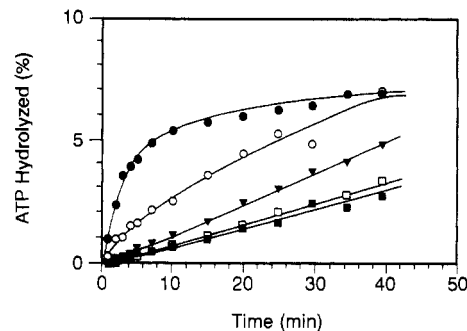
FIGURE 5: Effect of preincubation time in the presence of ADP on lag type kinetics. The concentrations of recA protein, poly(dT), ATP, and ADP are 5 \mu M, 10 \mu M, 2 mM, and 3 mM, respectively. RecA protein was preincubated with poly(dT) for 10 min before ADP was added. After incubation times of 0 (●), 1 (○), 5 (▼), 10 (□), and 30 (■) min, ATP was added to initiate the reaction.
