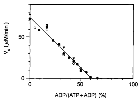
FIGURE 2: Effect of ADP on steady-state rates of poly(dT)-dependent ATP hydrolysis. Rates were taken from time courses such as those in Figure 1 and reflect either the initial rate of the reaction (at low ADP concentration) or an estimate of the rate observed after any transient phase was completed (at ADP/ATP ratios >0.4 ). RecA, poly(dT), and ATP concentrations were as in Figure 1. Different symbols reflect different protocols: (●) protocol of Figure 1A, (▼) protocol of Figure 1B, and (○) protocol of Figure 1A except that ADP was added 1 min after addition of ATP.
