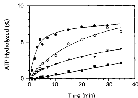
FIGURE 6: Effect of additional poly(dT) on the transient kinetic phase. Poly(dT) (10 \mu M) and 2 (■), 5 (▼), or 10 (○) \mu M recA protein were preincubated with ADP (3 mM). After 10 min, more poly(dT) (10 \mu M) and ATP (2 mM) were added to start the reaction. As a control to illustrate burst type kinetics for comparison purposes, poly(dT) (10 \mu M) and recA protein (5 \mu M) were preincubated, and then a mixture of ATP (2 mM) and ADP (3 mM) was added to start the reaction (●).
