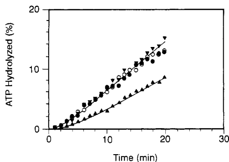
FIGURE 4: Effect of recA protein concentration on lag type kinetics. Poly(dT), ATP, and ADP concentrations were 10 \mu M, 2 mM, and 2 mM, respectively. The protocol of Figure 1B was used. RecA protein concentrations were as follows: (▲) 2 \mu M, (●) 5 \mu M, (○) 10 \mu M, and (▼) 20 \mu M.
