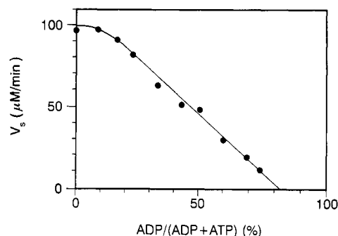
FIGURE 10: Effect of ADP on steady-state rates of high-salt-activated (DNA-independent) ATP hydrolysis. RecA protein and ATP concentrations were 5 \mu M and 2 mM, respectively. Data shown were obtained by preincubating recA protein for 10 min, and then initiating the reaction with a mixture of ATP and ADP.
